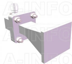
LB-75-10-C-TFSP Standard Gain Horn Antenna 10-15GHz 10dB Gain TNC Female
