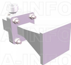
LB-75-10-C-NFSPO Standard Gain Horn Antenna 10-15GHz 10dB Gain N Type Female
